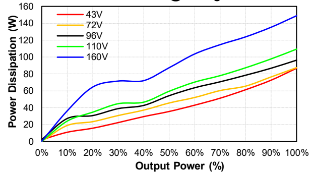
CFB600W-110S48-CMFD Pd Vs Po @25 Deg. C
