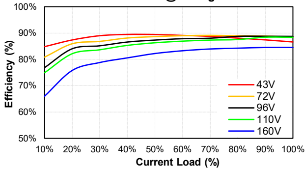
CF600W-110S28-CMFD Eff Vs Io @25 Deg. C
