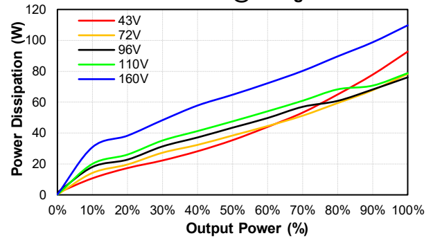
CFB600W-110S28-CMFD Pd Vs Po @25 Deg. C
