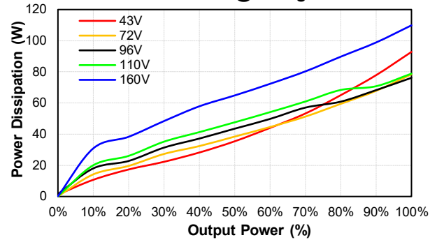
CFB600W-110S24-CMFD Pd Vs Po @25 Deg. C
