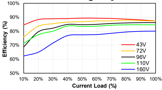
CF600W-110S48-CMFD Eff Vs Io @25 Deg. C
