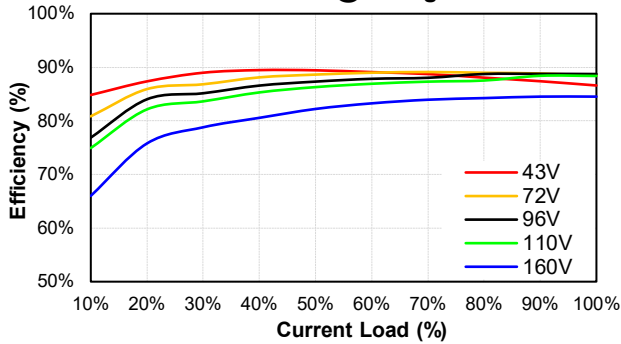
CF600W-110S24-CMFD Eff Vs Io @25 Deg. C
