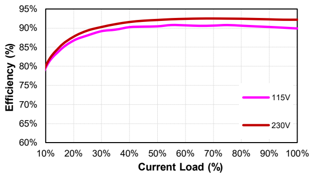
CFM300S120 (Eff Vs Io)
