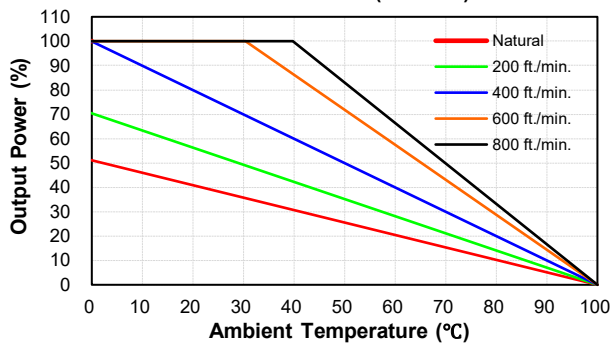
CHB150W8-36S Derating Curve without Heatsink (Vin=36V)
