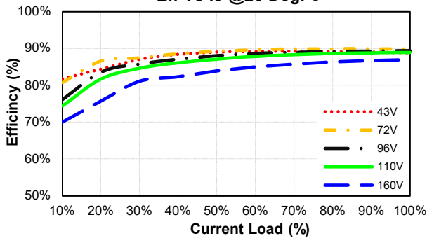
CHB200W-110S24 Eff Vs Io @25 Deg. C
