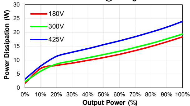
CQB150-300S24-CMFC Pd Vs Po @25 Deg. C
