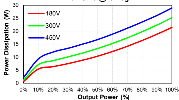
CQB150-300S05-CMFC Pd Vs Po @25 Deg. C
