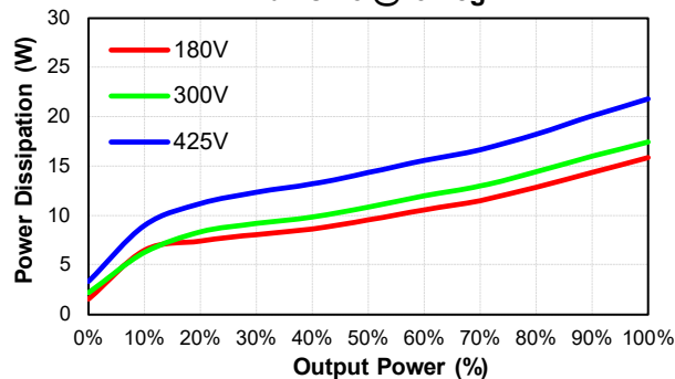
CQB150-300S15-CMFC Pd Vs Po @25 Deg. C
