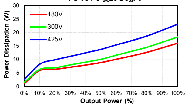
CQB150-300S12-CMFC Pd Vs Po @25 Deg. C
