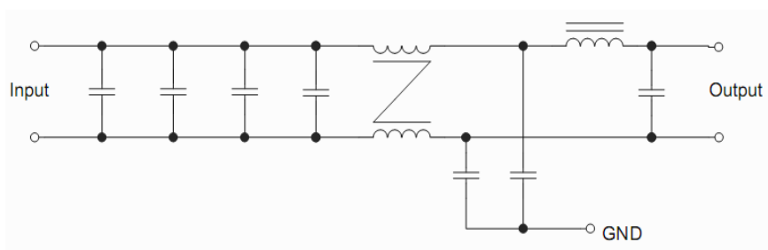
Figure1 Internal Schematic for FM10-100 Module
