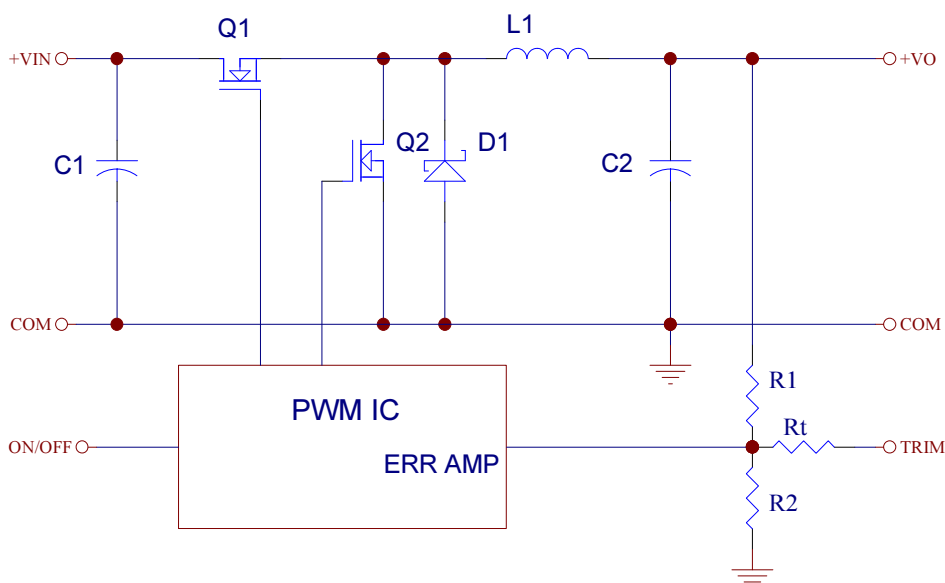
Figure 1. Simplified Schematic
